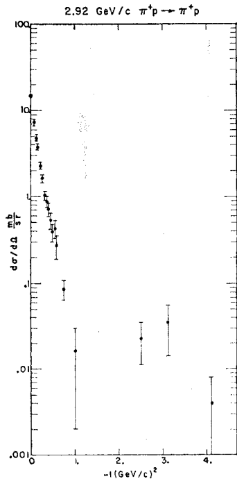
FIG. 6. Elastic scattering differential cross sections for 2.92-GeV/c \pi^+p . The error's shown are statistical. An additional normalization uncertainty of \frac{+30\%}{-10\%} , is not indicated. The open circle at t=0 is the optical theorem prediction.
