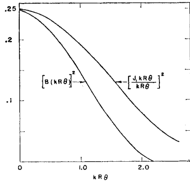
FIG. 1. The functions [J_1(kR\theta)/kR\theta]^2 and [B(kR\theta)]^2 versus kR\theta .
