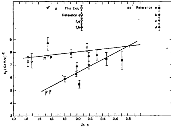
FIG. 17. The coefficient A_1(\text{GeV}/c)^{-2} versus \ln s from linear fits to pp and \pi p elastic-scattering data according to d\sigma/d\Omega = \exp(A_0 + A_1 t) in the range 0 < |t| < 0.4 ( \text{GeV}/c ) 2 . The straight lines are fitted to the plotted points for pp and \pi p scattering considered separately.
